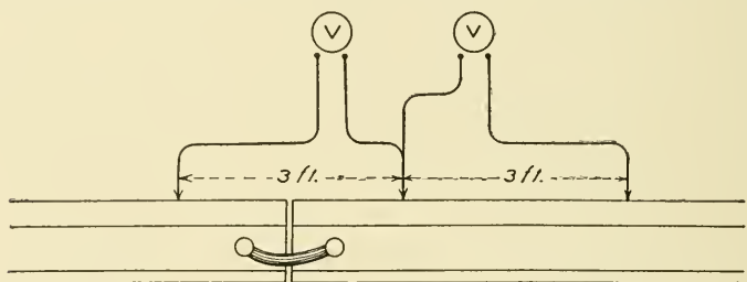
Fig. 207. Common Form of Bonded Joint with Milli-Voltmeters Attached to Show Voltage Drop
